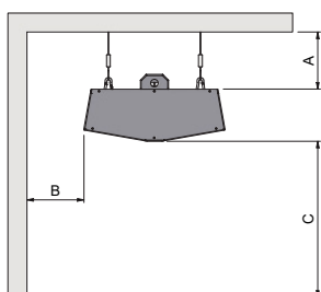
HANGING 3200 / 6400
