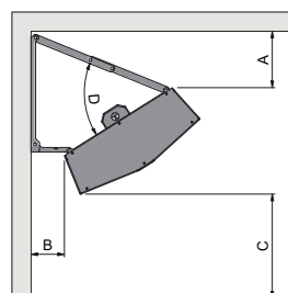
WALL BRACKETS 3200 / 6400
